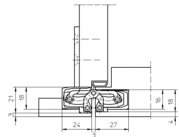
Futterzarge
